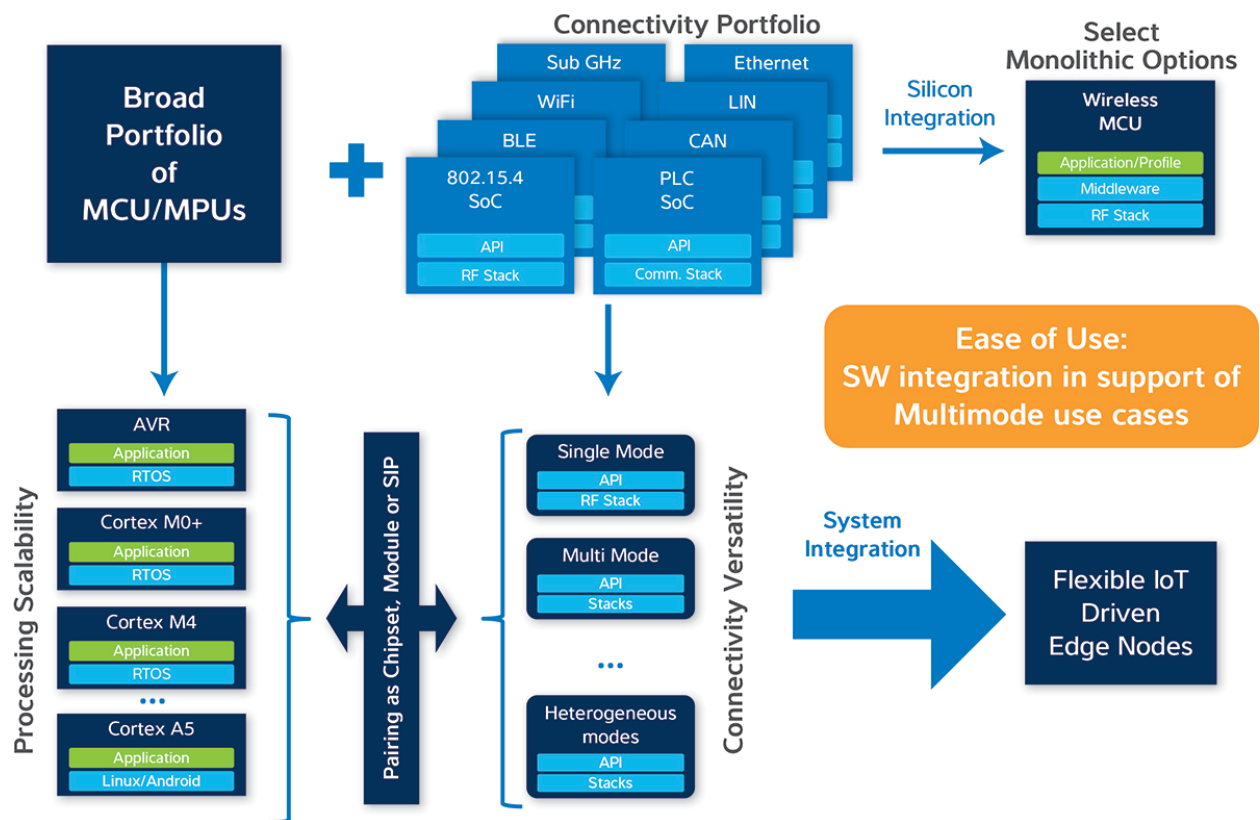
Figure 7 – The Atmel SmartConnect connectivity approach
