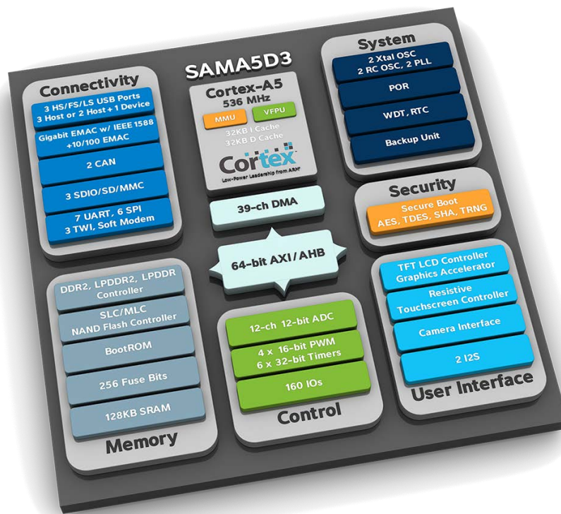
Figure 5 – The Atmel SAMA5D3 device block diagram
