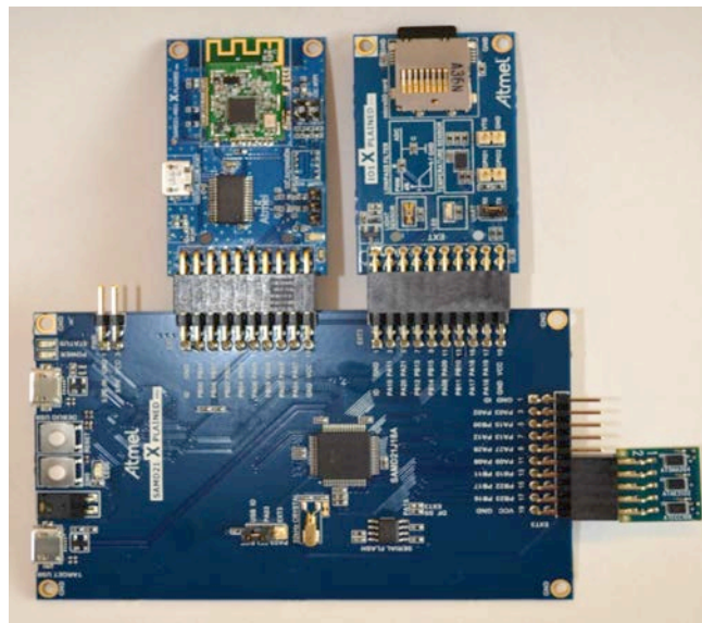
Figure 6 – SAM D21 Xplained Pro demo board with temp sensor, WiFi, and CryptoAuthentication modules connected
